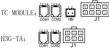
SKETCH OF INTERFACE PIN:
